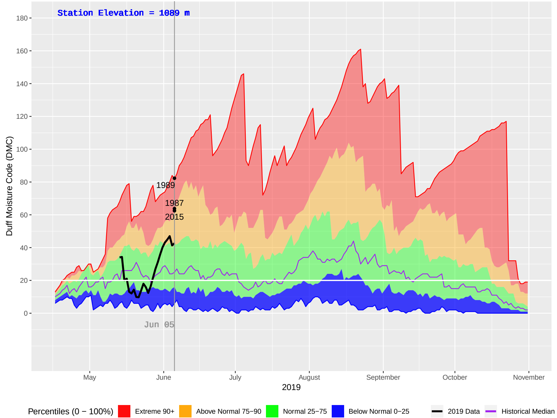
EAST OOTSA (170) : Historical (1986–2018), Current (2019) Daily Duff Moisture Code (DMC)
