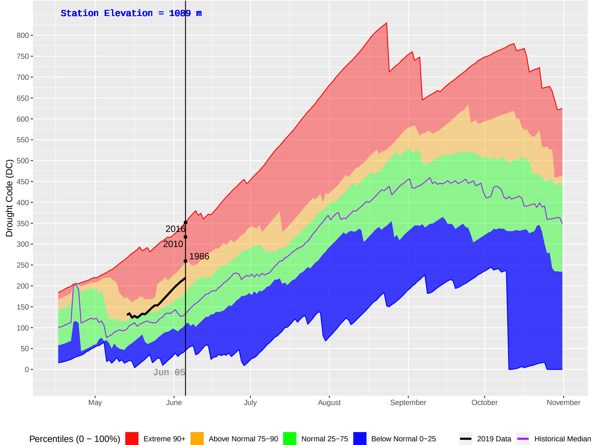
EAST OOTSA (170) : Historical (1986–2018) and Current (2019) Daily Drought Code (DC)
