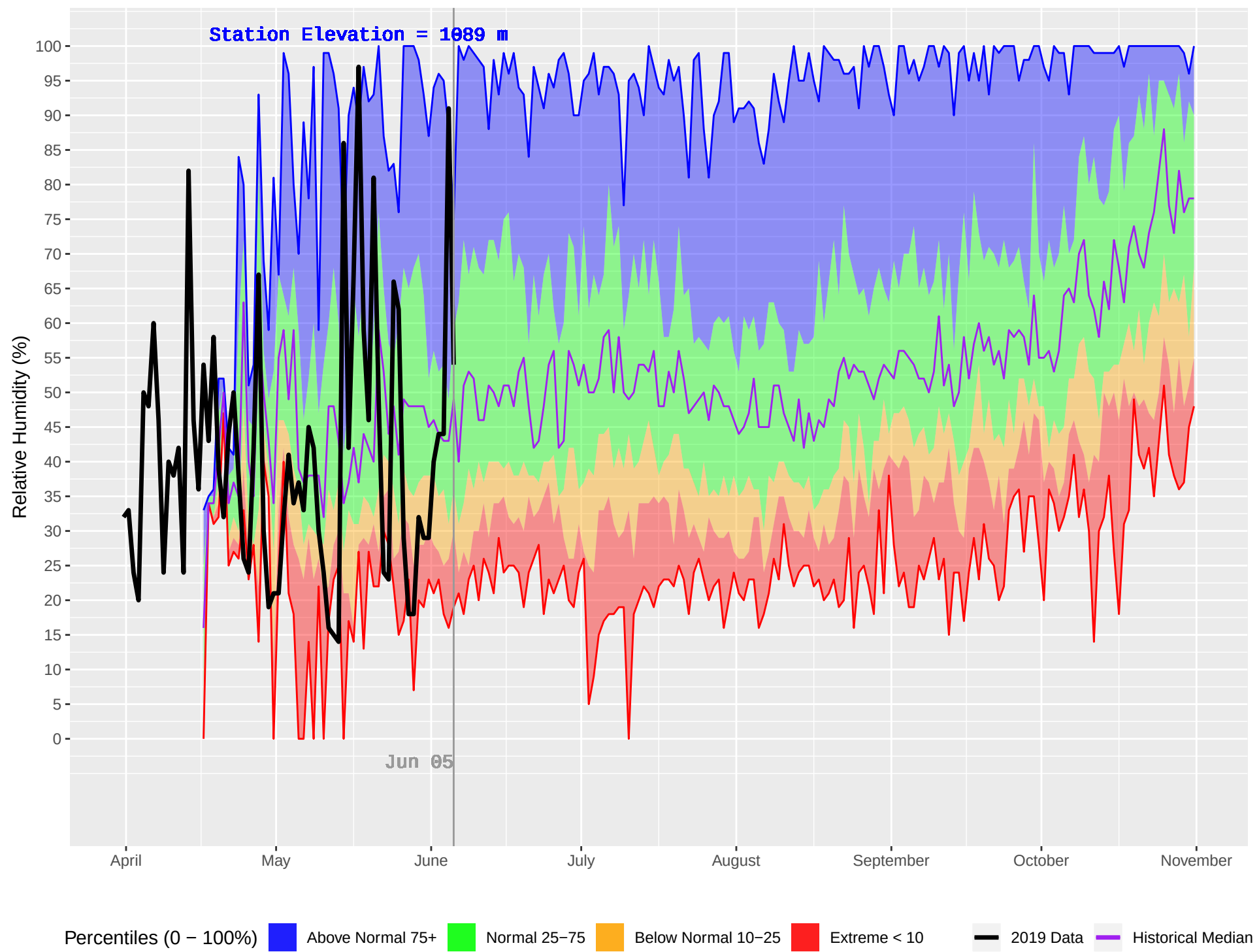
EAST OOTSA (170) : Historical (1986–2018) and Current (2019) Daily Relative Humidity
