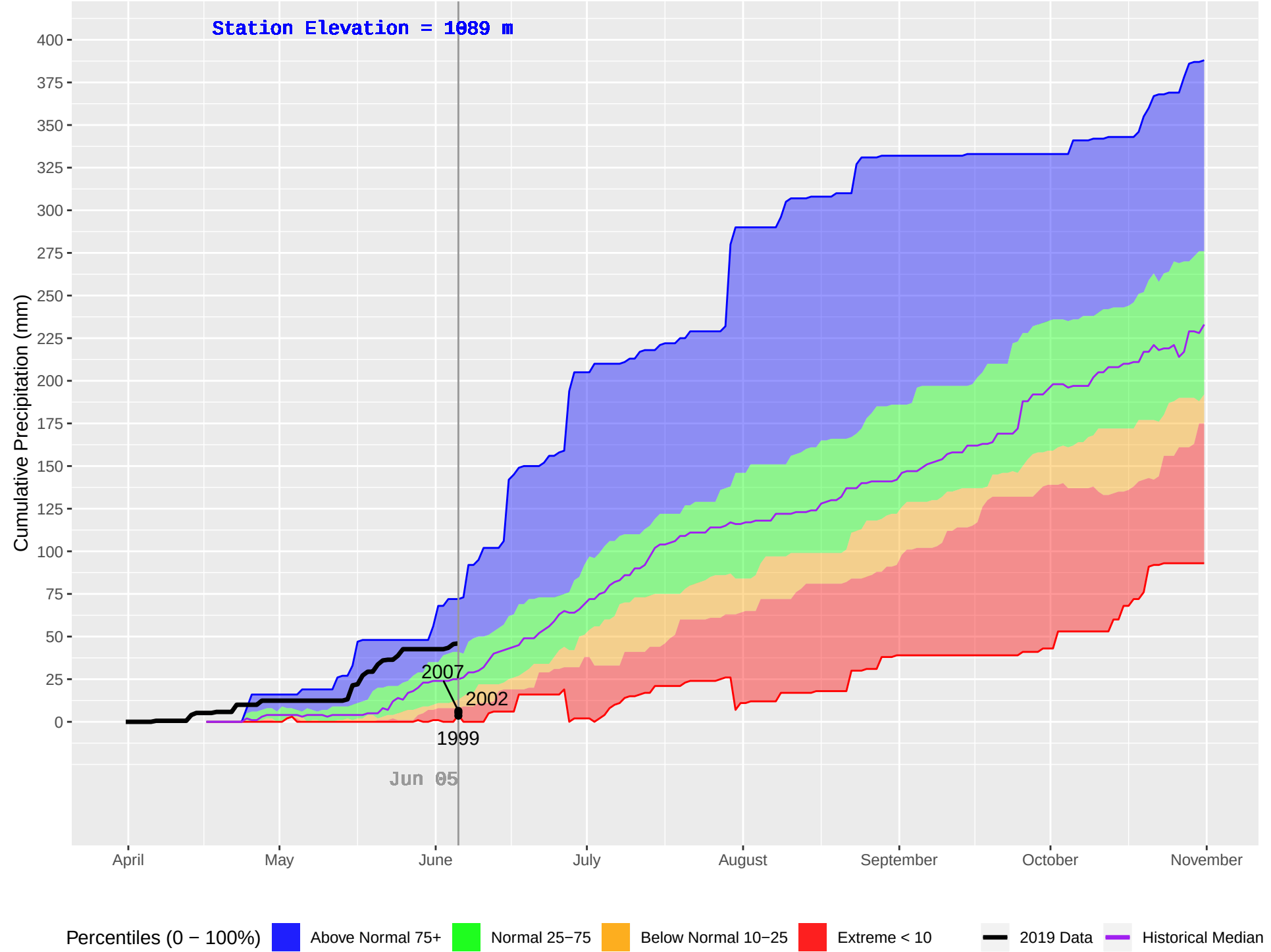
EAST OOTSA (170) : Historical (1986–2018), Current (2019) Daily Cumulative Precipitation
