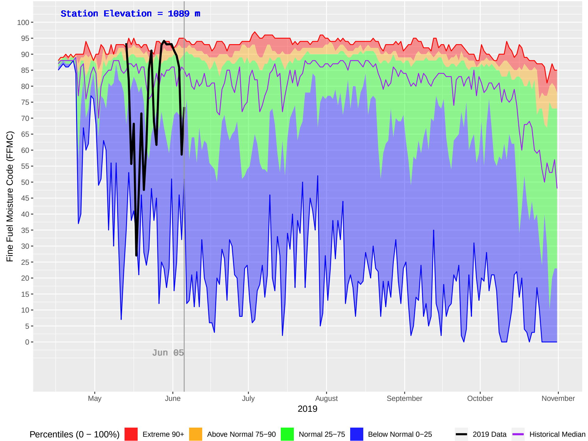
EAST OOTSA (170) : Historical (1986–2018) and Current (2019) Daily Fine Fuel Moisture Code (FFMC)
