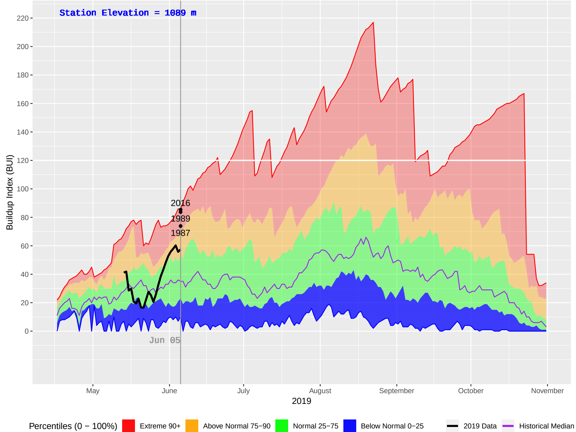
EAST OOTSA (170) : Historical (1986–2018), Current (2019) Daily Buildup Index (BUI)
